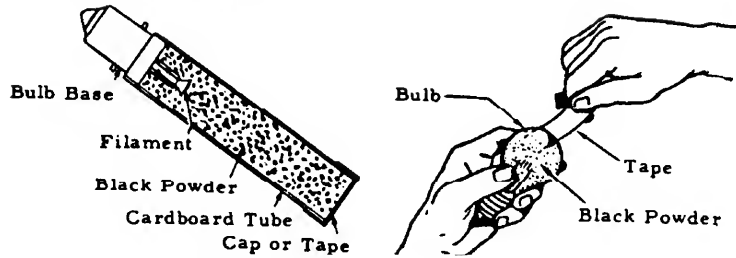
CARDBOARD TUBE DEVICE
